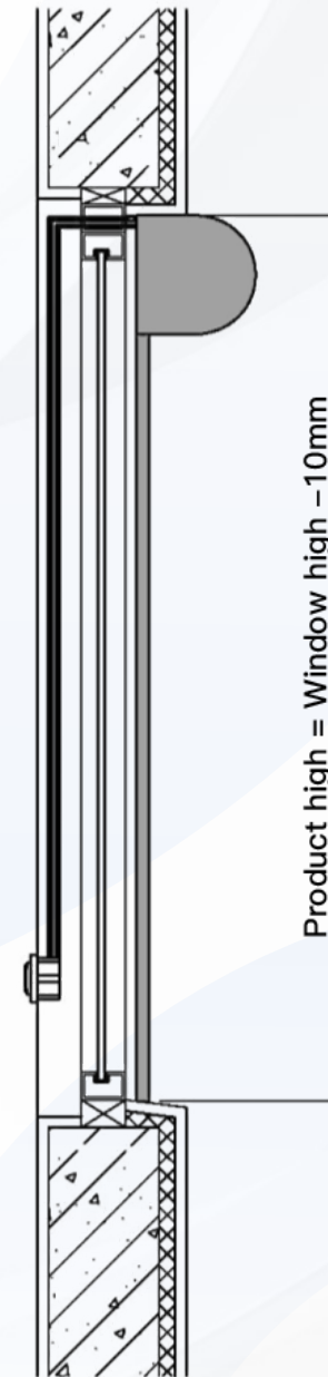
In-window installation
